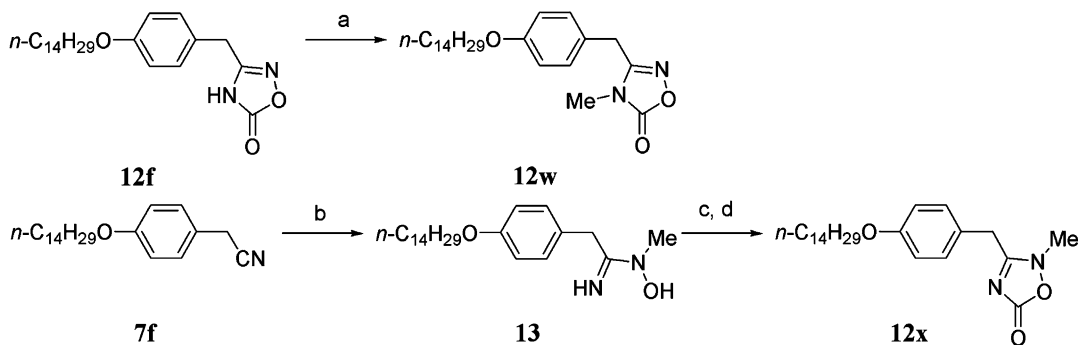
Scheme 5. Reagents and conditions: (a) \text{CH}_2\text{N}_2/\text{ether} , \text{K}_2\text{CO}_3 , DMF; (b) \text{MeNHOH}\cdot\text{HCl} , \text{K}_2\text{CO}_3 , abs EtOH; (c) \text{ClCOOEt} , \text{Et}_3\text{N} , \text{CH}_2\text{Cl}_2 ; (d) toluene, reflux.
